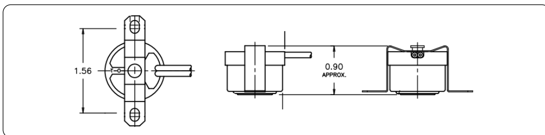
FIG 15A. THERMO DISC DETAIL
