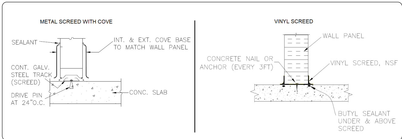
FIG 5. FLOOR SCREED
