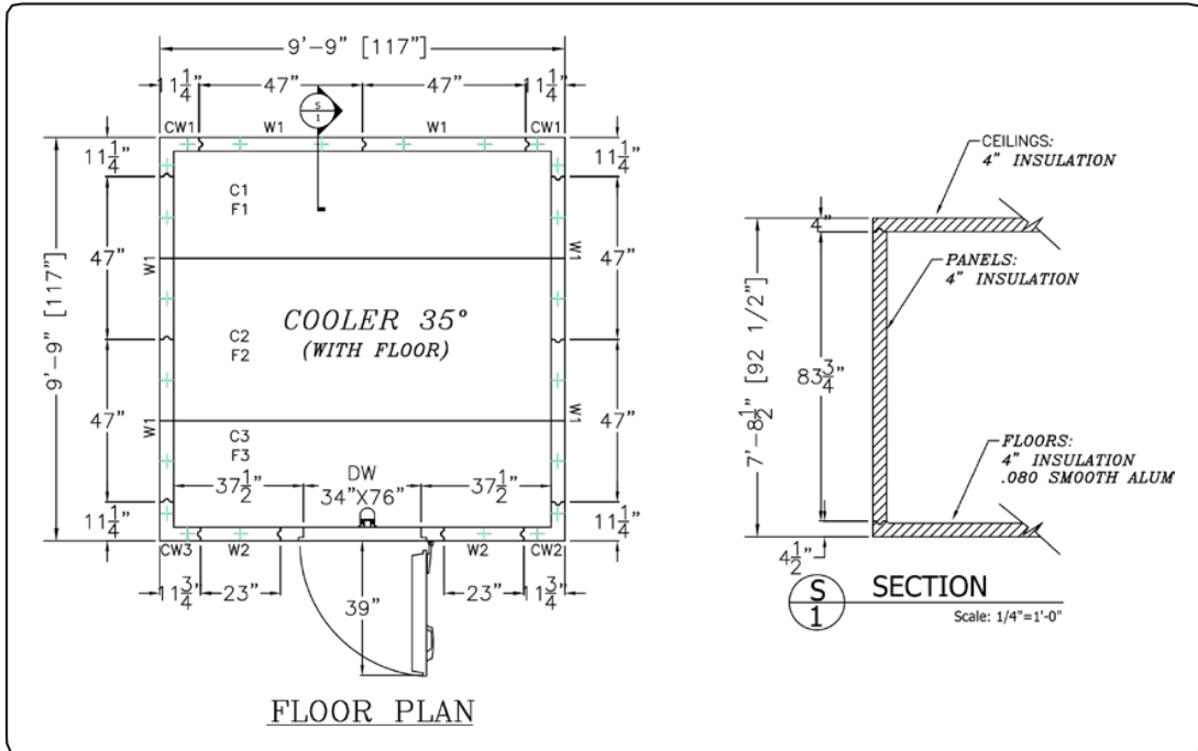
FIG 1. LAYOUT DRAWING
