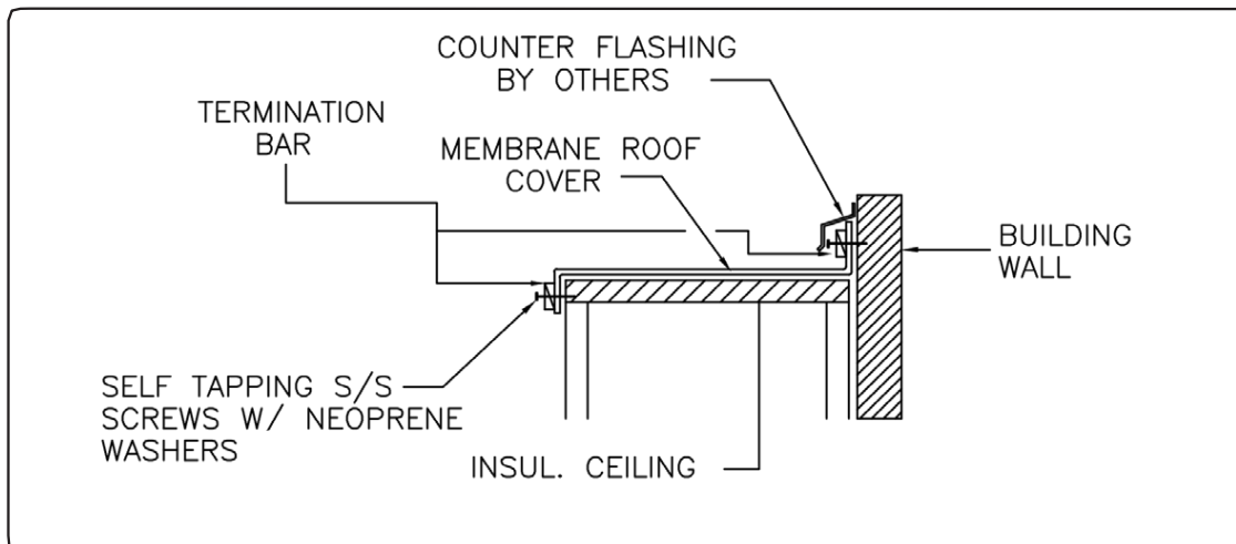
FIG 11. TYPICAL MEMBRANE COVER INSTALLATION WITH ADJACENT WALL
