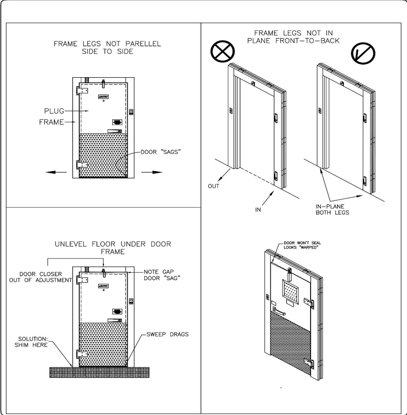
FIG 8. INSTALLATION DOOR PROBLEMS
