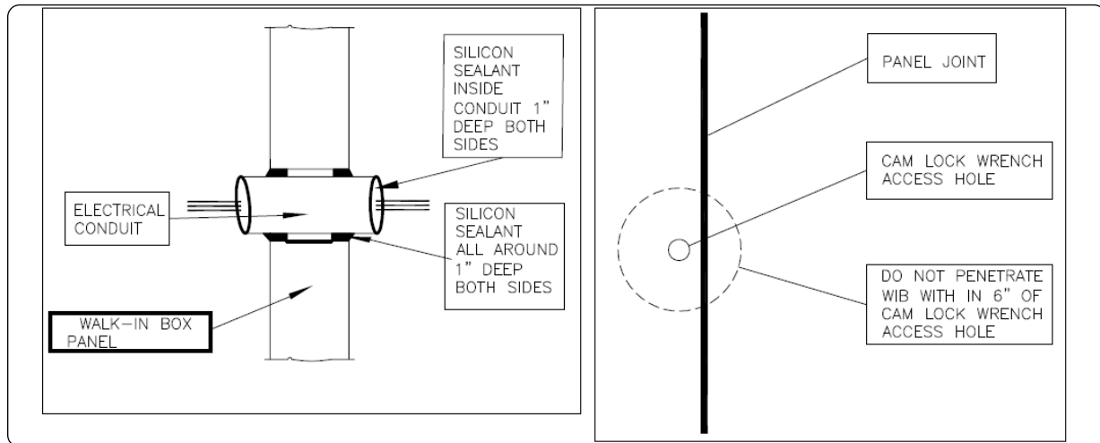
FIG 15. SEALING OF WALK-IN ELECTRICAL PENETRATIONS
